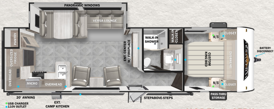
MODEL #: 27RK HITCH: 955 LBS UVW: 6,863 LBS LENGTH: 33'6"
